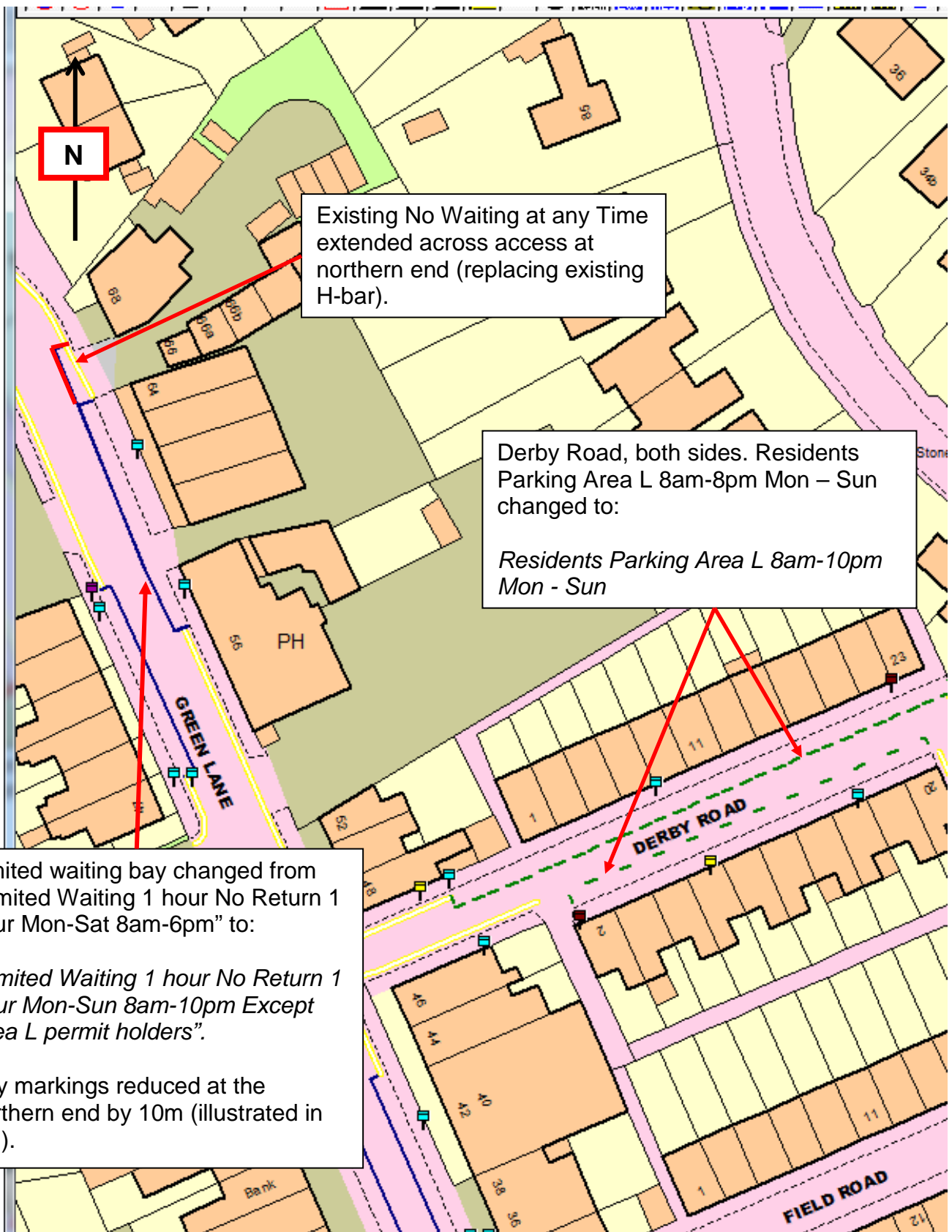
Drawing E8935 – Sheet 4 of 4 – APPROVAL REQUESTED TO ADVERTISE
