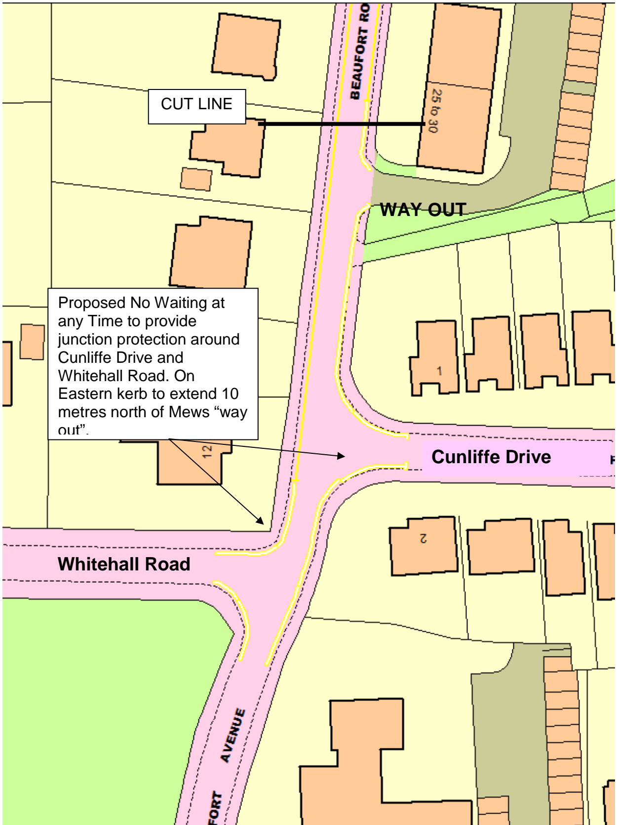
Drawing E8924 – Sheet 4 of 4
