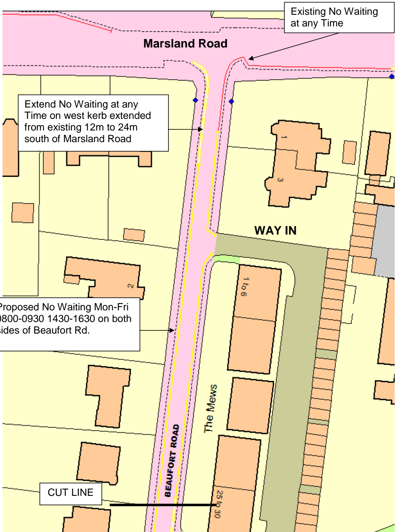
Drawing E8924 – Sheet 3 of 4 Existing restrictions indicated in red.
